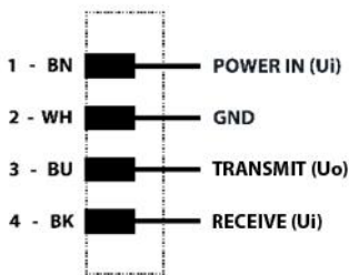
Diagram 15.4.2 Power port circuit diagram Contact assignment of the M12 plug and M12 receptacles
